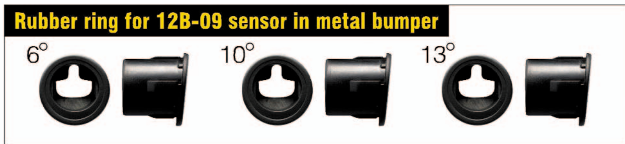
Snap-on angle rings for SM-12B-09 sensors
