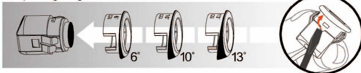
Snap-on angle rings for SM-12B-09 sensors
